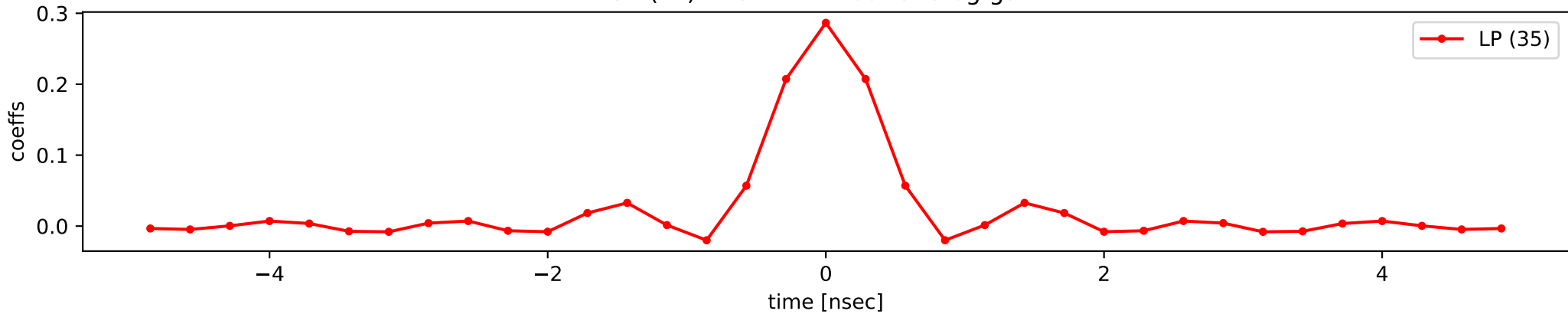
S4 (LP) ver2 without analog gain
