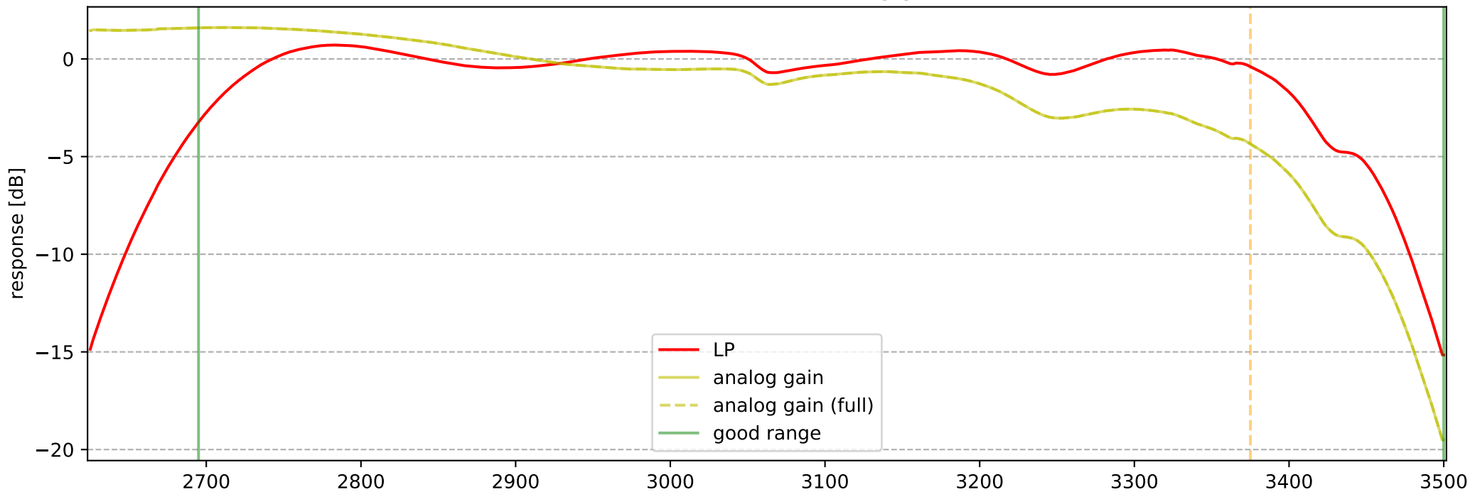
S4 (LP) ver2 with analog gain
