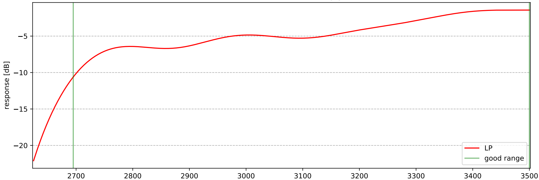
S4 (LP) ver2 without analog gain
