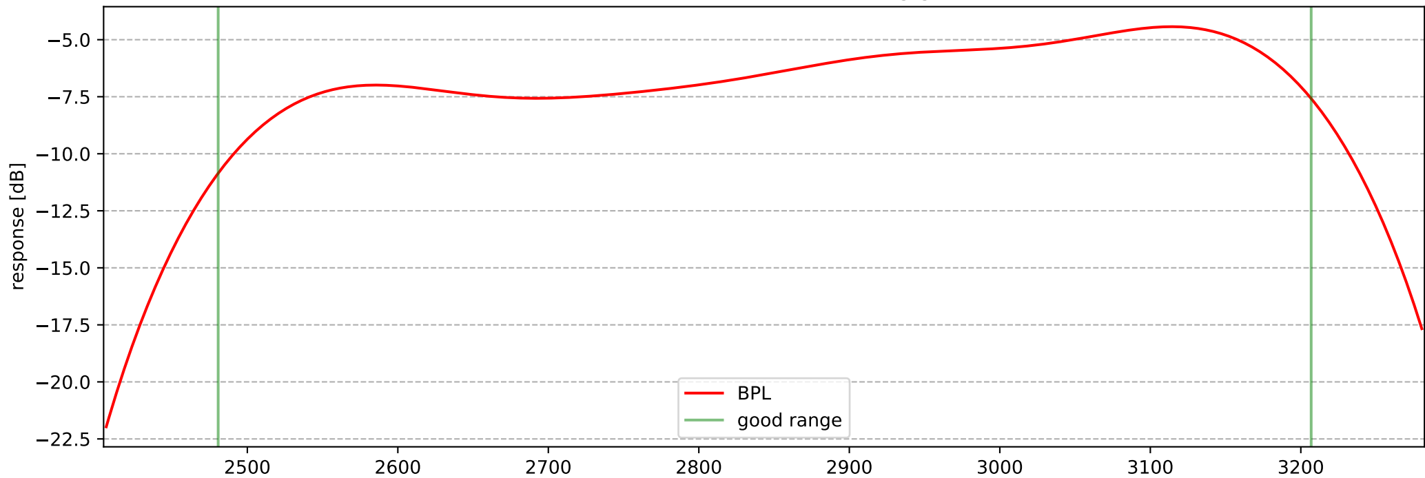
S3 (BPL) ver2 without analog gain
