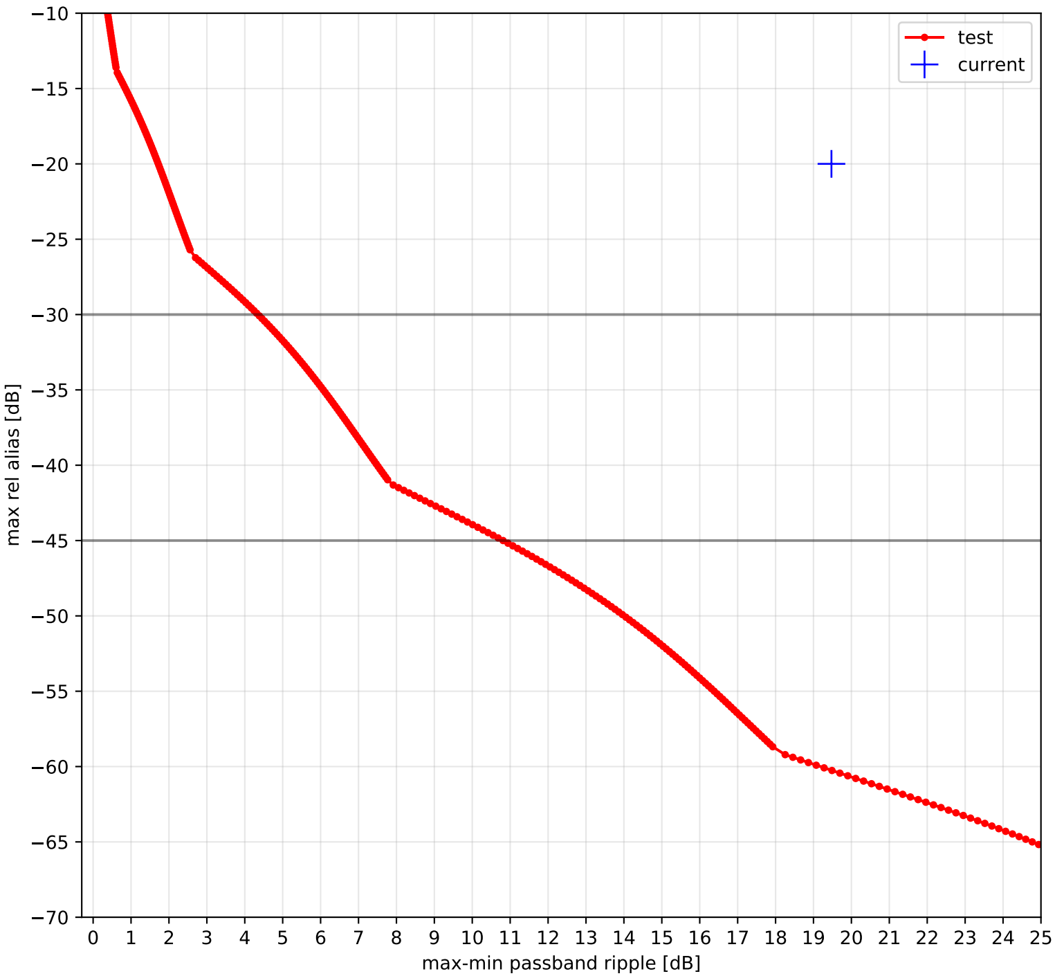
usable bandwidth 95.000 %
