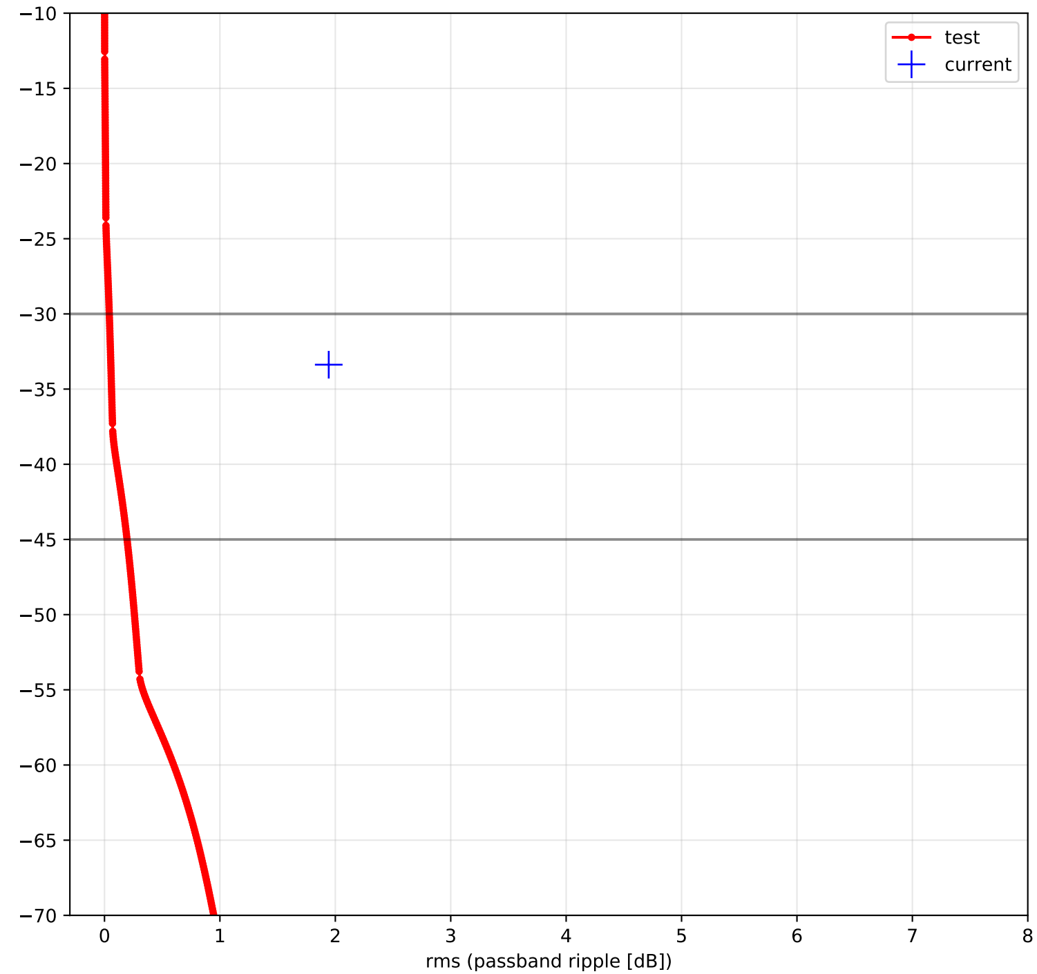
usable bandwidth 90.500 %
