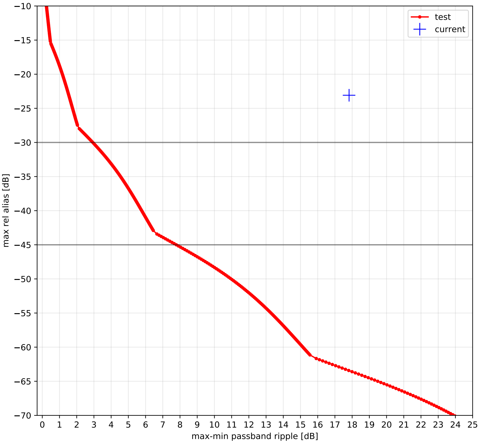
usable bandwidth 94.250 %
