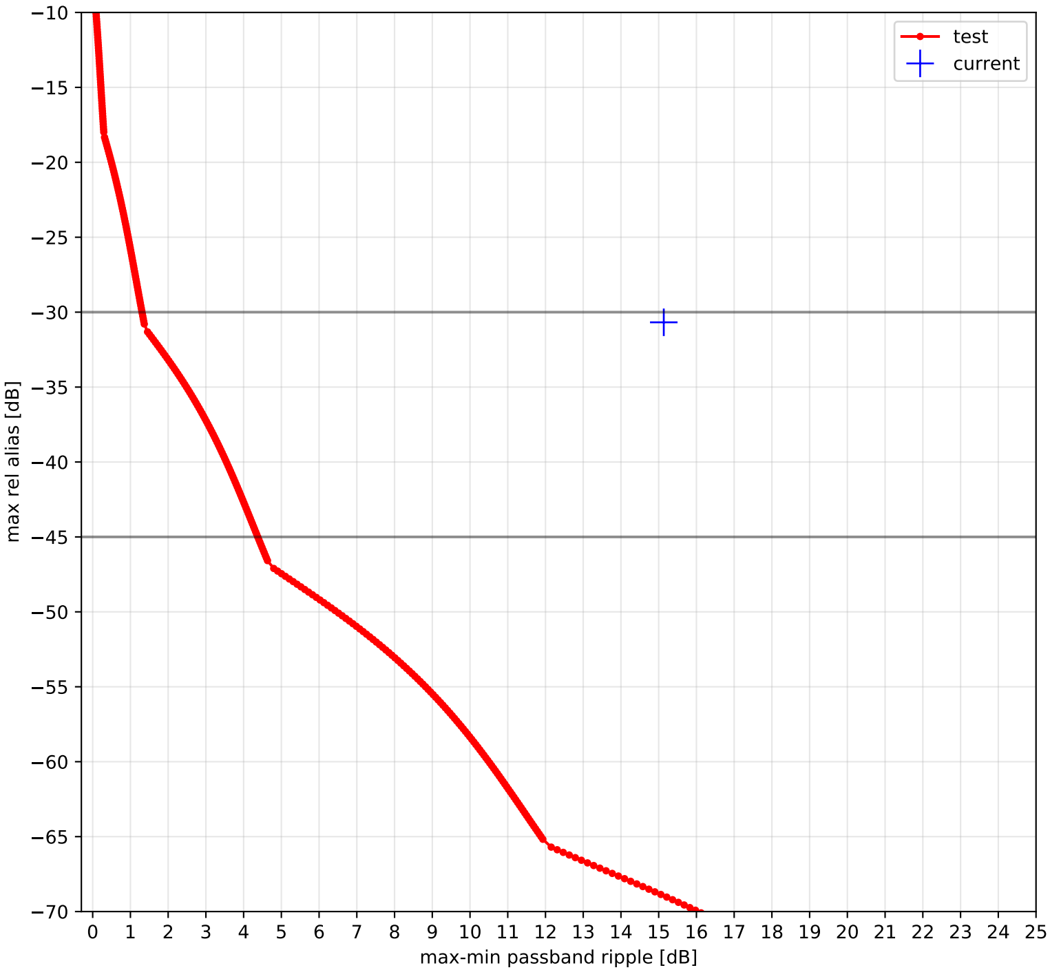
usable bandwidth 93.000 %
