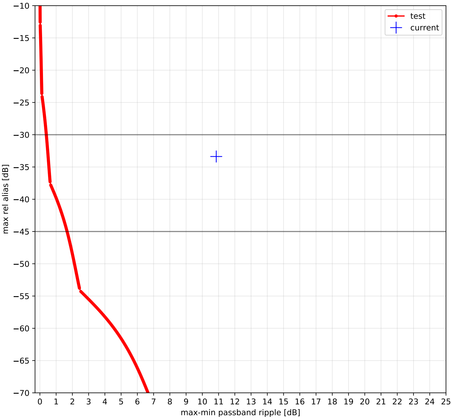
usable bandwidth 90.500 %
