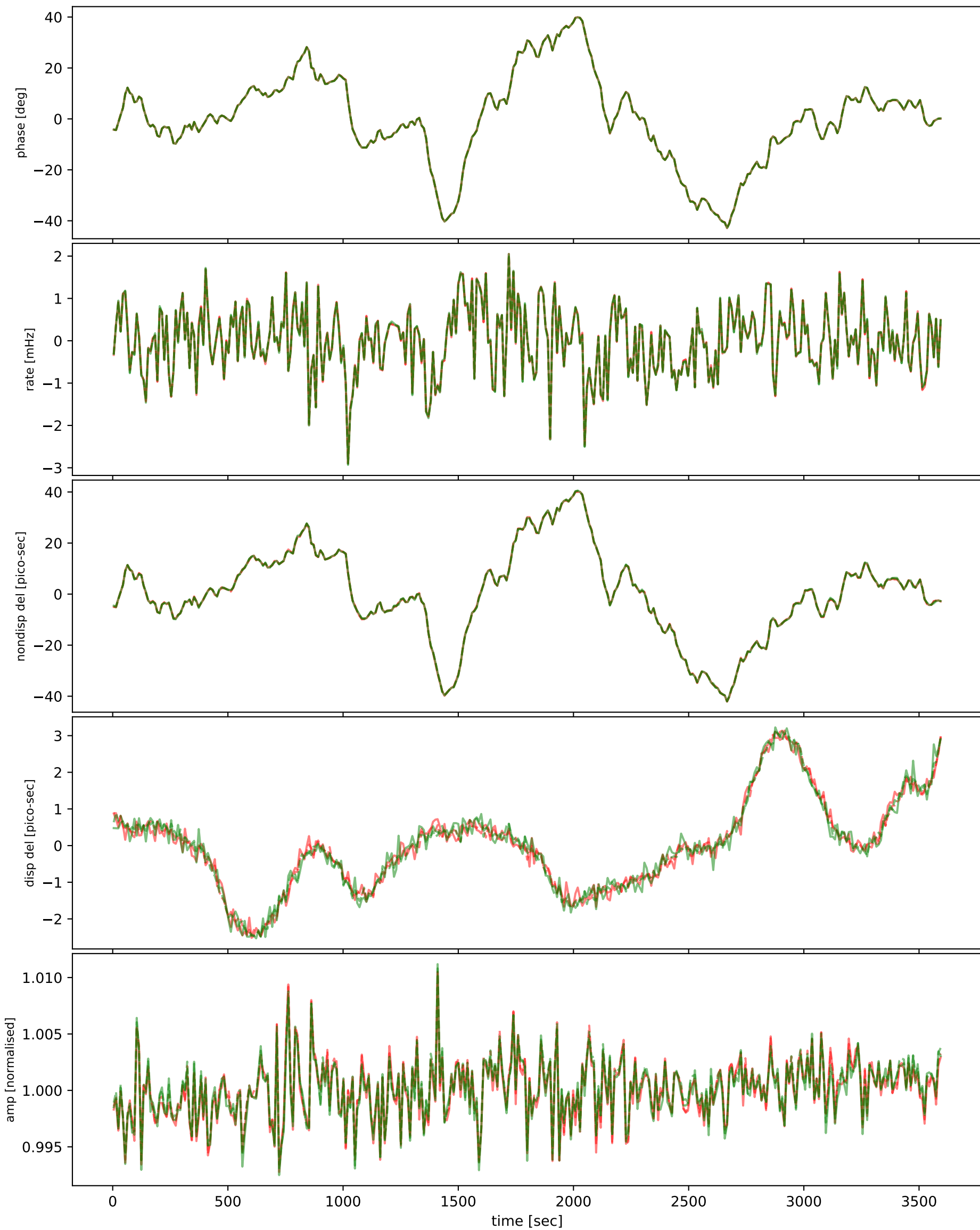
m045-m057
