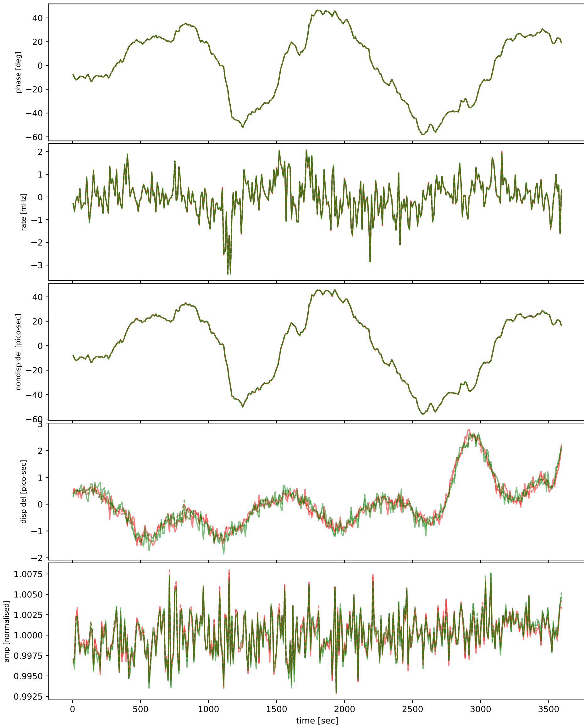
m002-m057
