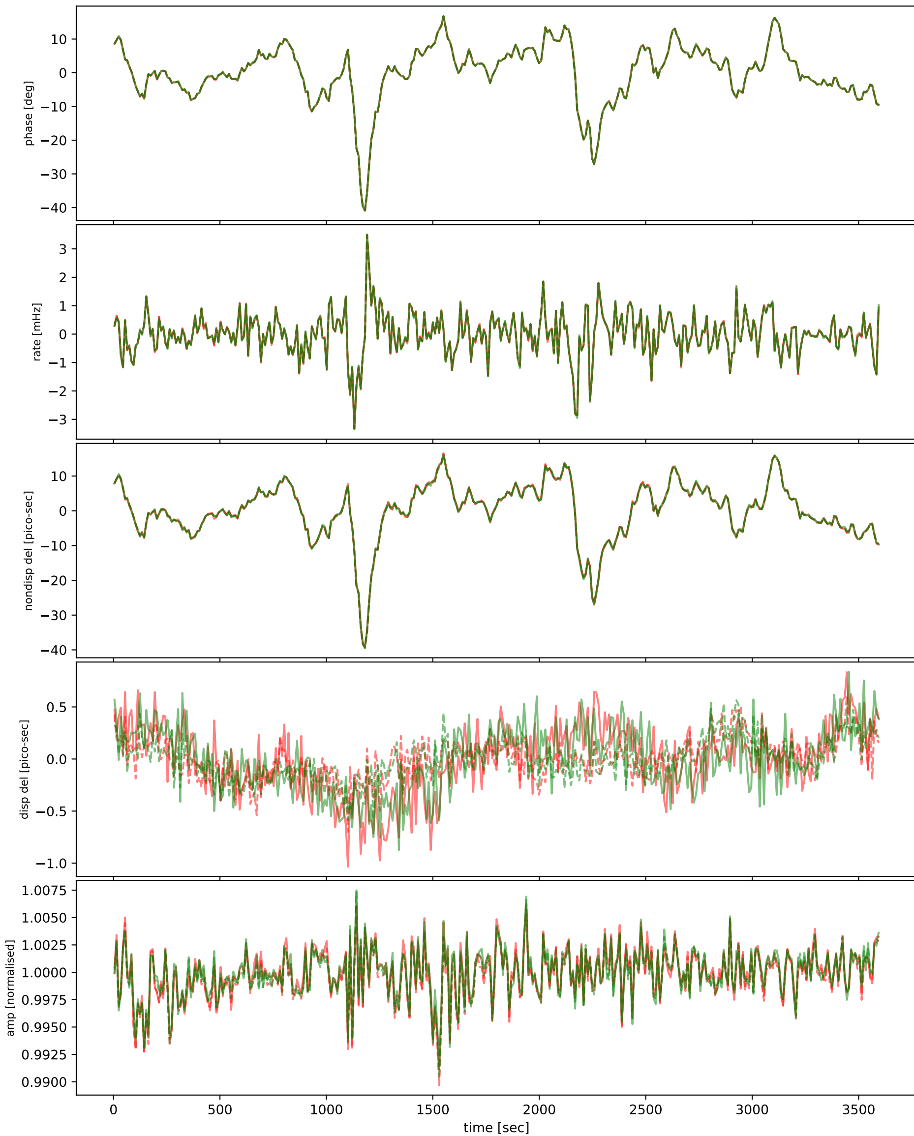
m006-m030
