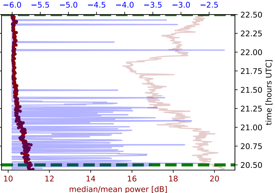
\log_{10} (incompleteness)
