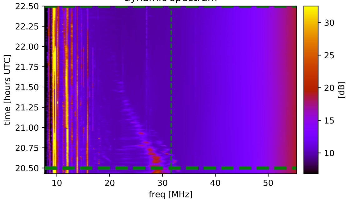
dynamic spectrum
