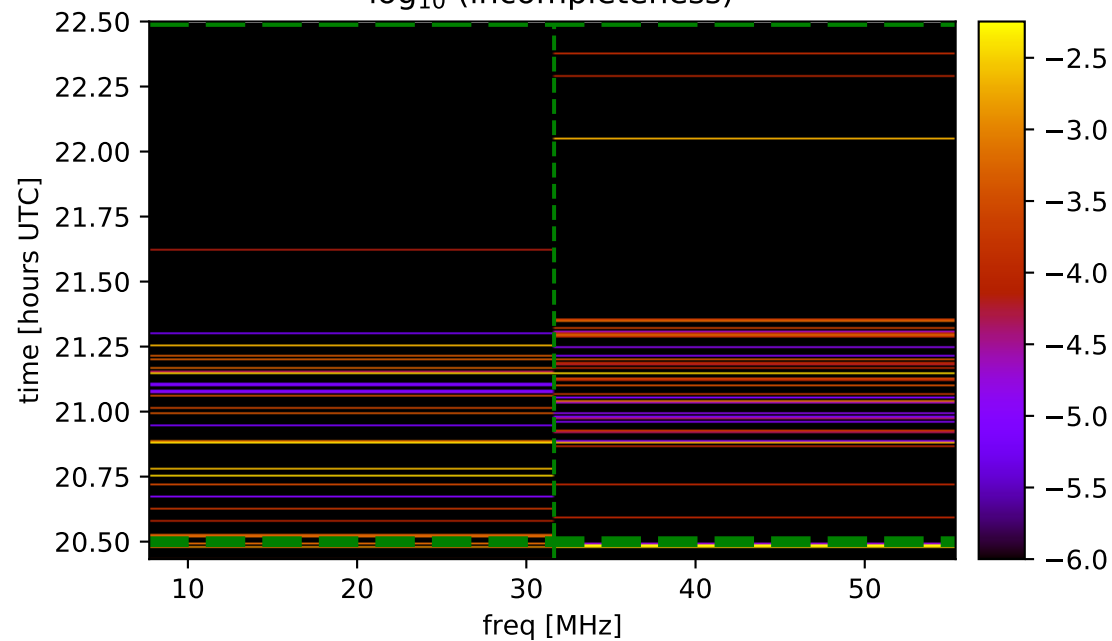
\log_{10} (incompleteness)
