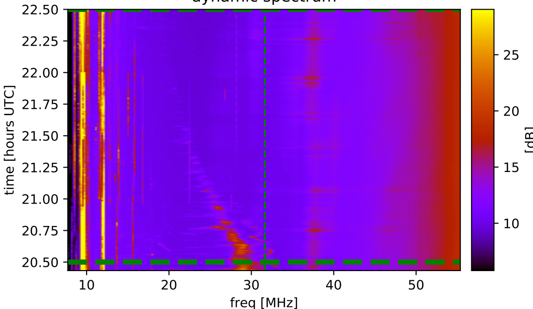
dynamic spectrum
