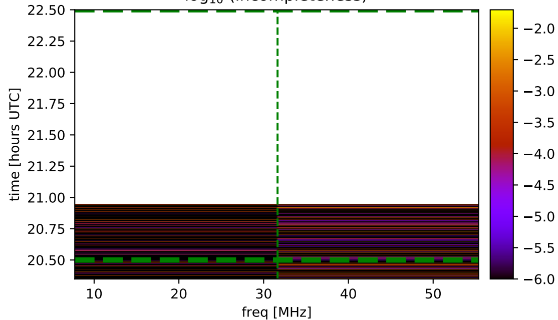
\log_{10} (incompleteness)
