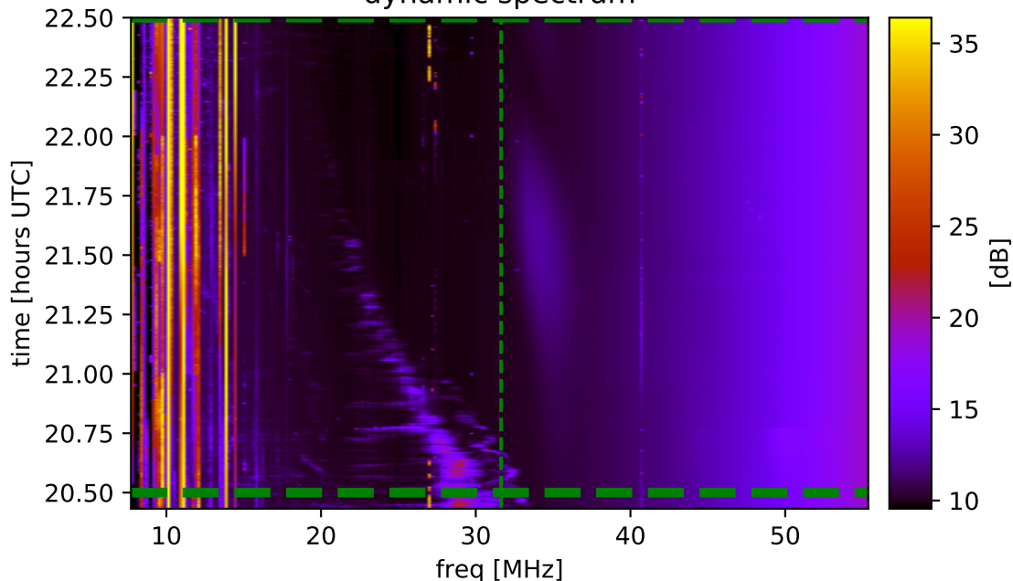
dynamic spectrum
