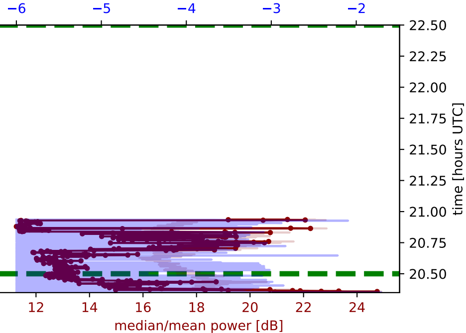
\log_{10} (incompleteness)
