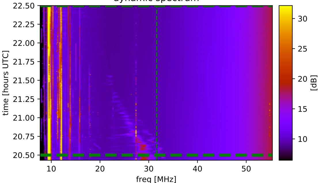
dynamic spectrum
