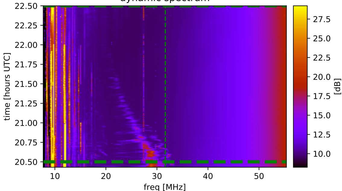
dynamic spectrum
