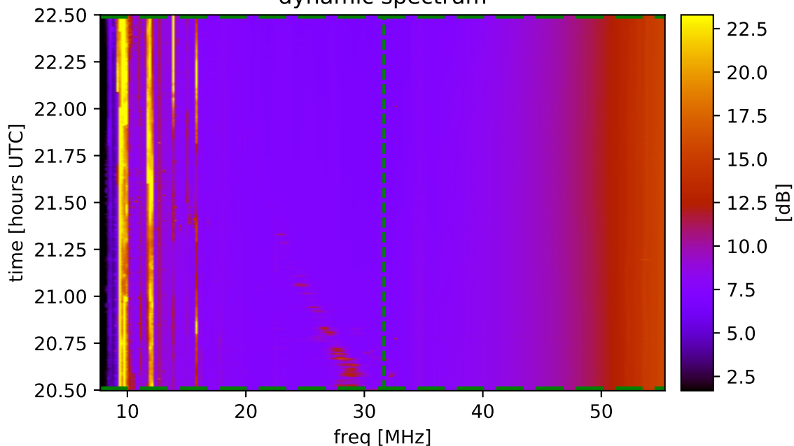
dynamic spectrum
