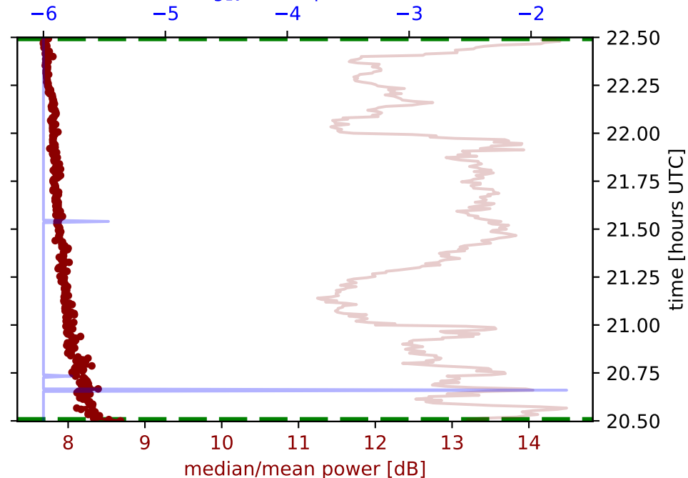
\log_{10} (incompleteness)
