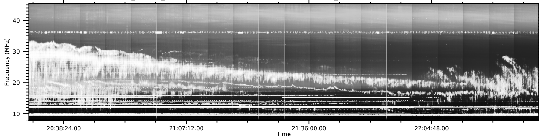
20231227_202900_BST - NW - Beam ana: 0 - Beam num: 0 - JUPITER_TRACKING - histogram-equalized data
