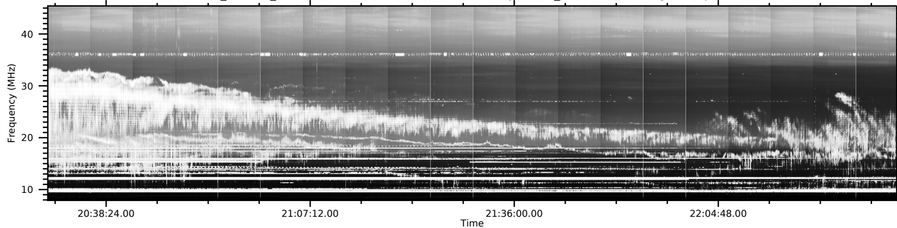
20231227_202900_BST - NE - Beam ana: 0 - Beam num: 0 - JUPITER_TRACKING - histogram-equalized data
